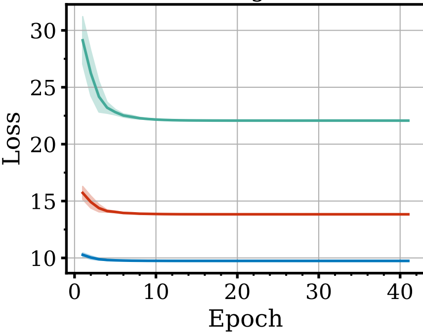
Training Loss
