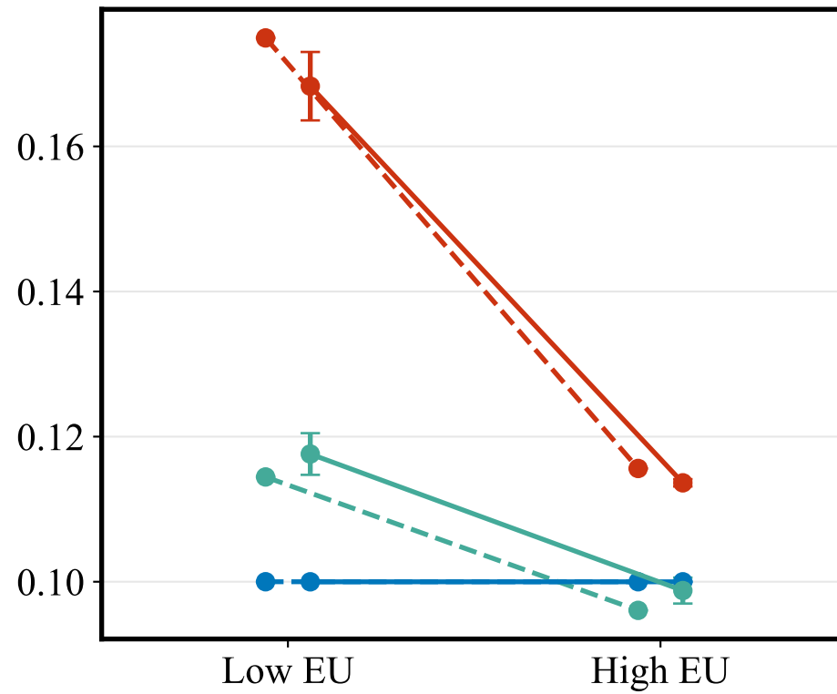
Mean \tilde{\alpha}
