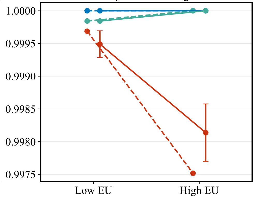
Empirical coverage
