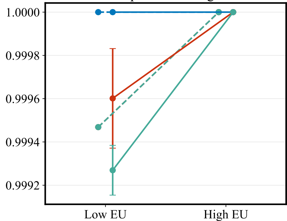
Empirical coverage
