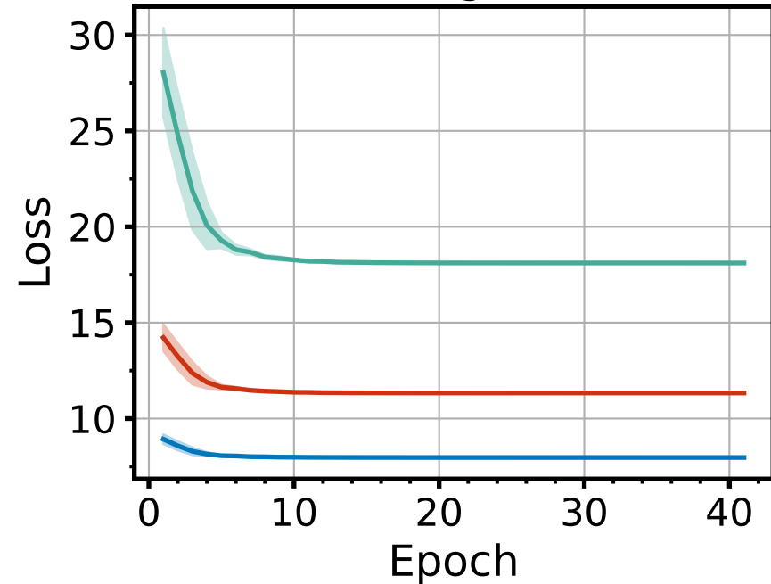
Training Loss
