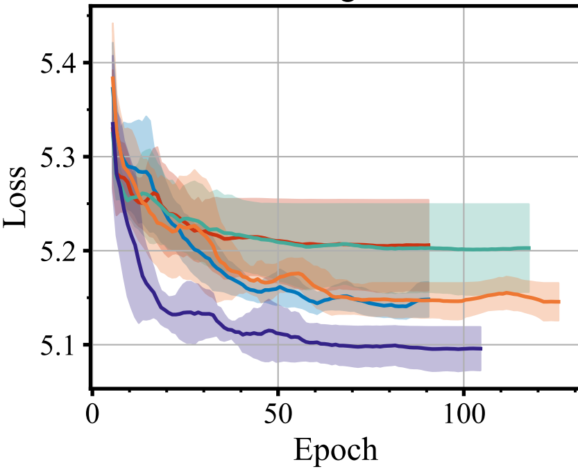
Training Loss
