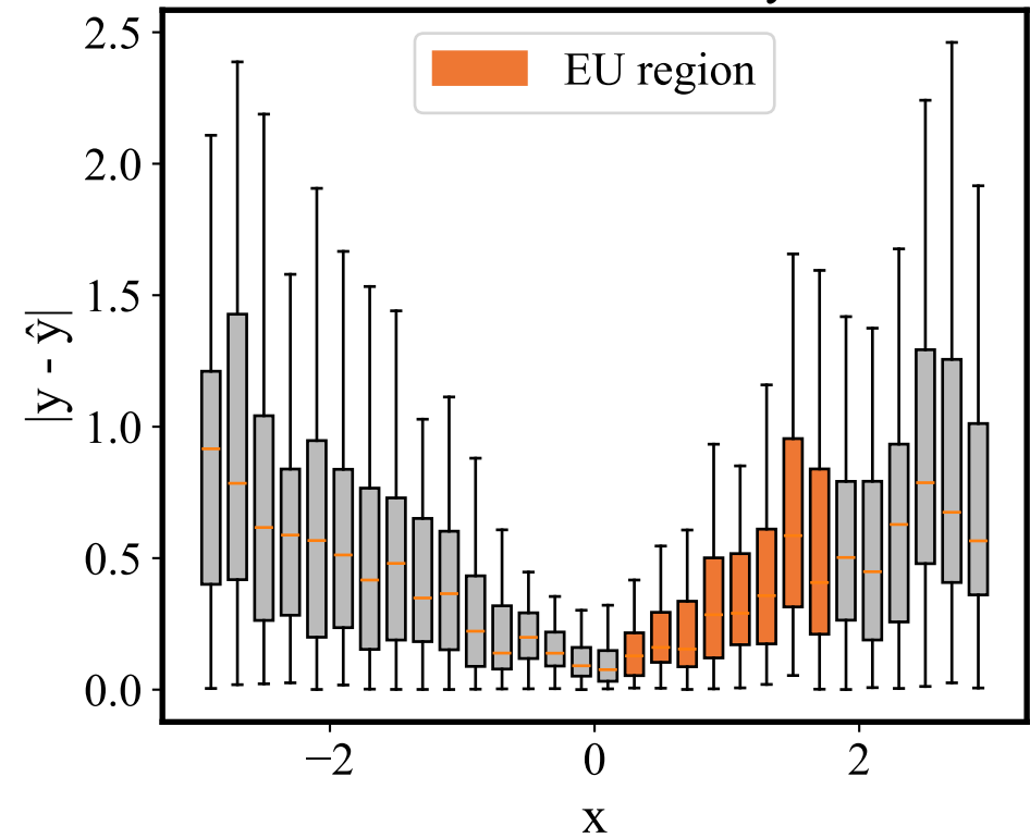
Absolute residual by x
