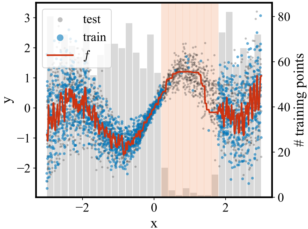
Data and fitted model
