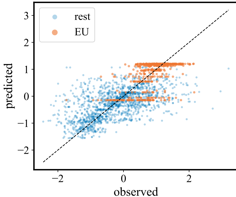
Predicted vs observed
