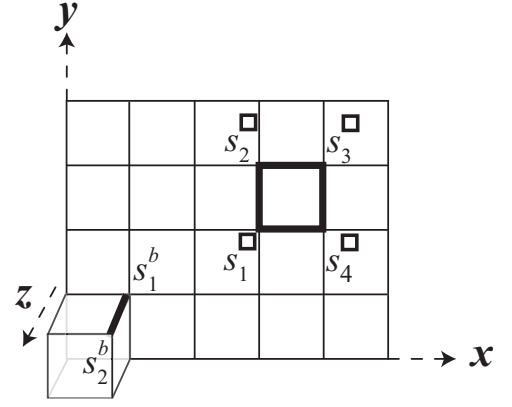
FIG. 1: The classical anisotropic 3D problem that describes the quantum critical point of the model (2). The two types of interactions (shaded bonds) are plaquette interactions in the planes normal to \hat{z} , and bond interactions along \hat{z} .
