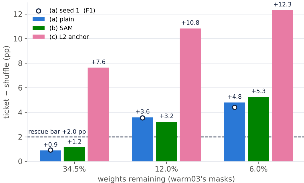
Figure 3. Ticket – shuffle advantage on warm03's three masks, trained at \eta = 0.1 without warmup. Dashed line: the pre-registered +2.0 pp rescue bar. Open circles: (a) repeated on seed 1 (F1, $4.5).
