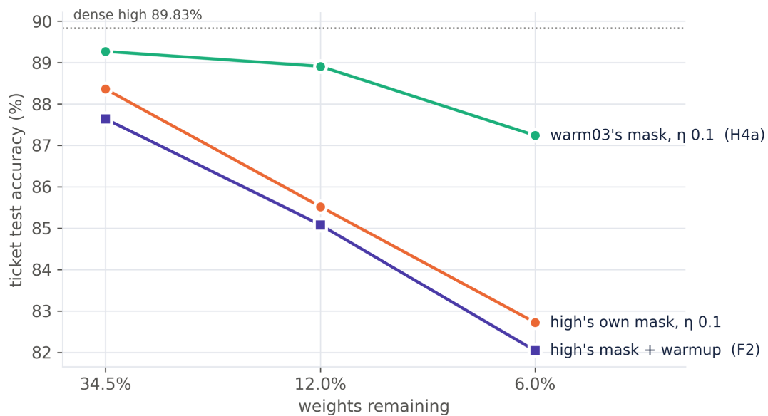
Figure 4. Ticket accuracy on three masks under the same training. The green and orange lines differ only in the mask (same \theta_0 , \eta = 0.1 , no warmup); the orange and violet lines differ only in warmup (F2, §4.5). The mask decides.
