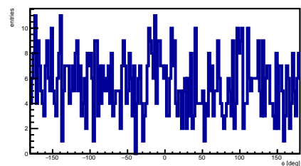
K + azimuth
