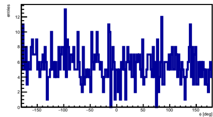
K - azimuth
