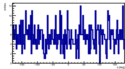
e' azimuth
