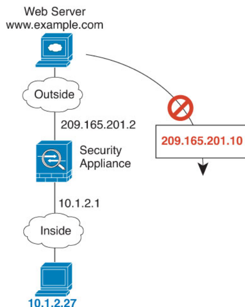
Figure 17: Remote Host Attempts to Initiate a Connection to a Mapped Address
