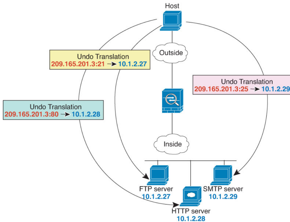
Figure 27: Static NAT-with-Port-Translation
