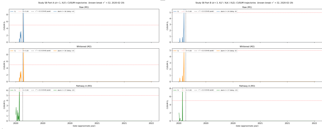
Figure 4. Study ETF: CUSUM trajectories on the COVID test window (2020-01-01 to 2022-06-30); the vertical dashed line marks \tau^* = 32 (2020-02-19). Left (Part A, d = 1 , XLF): the Innovation CUSUM (bottom) crosses threshold h = 5 at t = 17 , fifteen steps before the official market peak. Right (Part B, d = 3 , XLF/XLK/XLE): the Innovation CUSUM again alarms at t = 17 , and its \text{ARL}_0 gap over M1/M2 widens relative to Part A, consistent with the dimension-stability prediction of Corollary 3.11.
