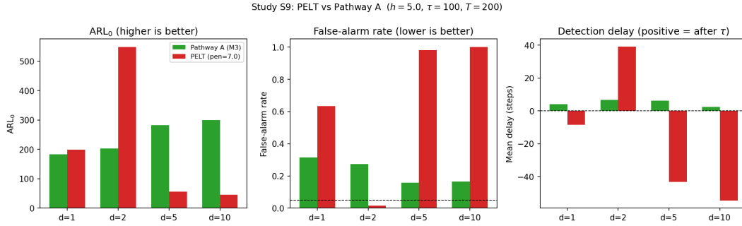
Figure D.4. Study PELT: \text{ARL}_0 (left), false-alarm rate (middle), and mean detection delay (right) for PELT (red) and the Innovation CUSUM (green) across d \in \{1, 2, 5, 10\} . PELT’s behavior is non-monotone in d : it alternates between over-conservatism ( d = 2 , near-zero detection) and under-conservatism ( d \geq 5 , near-100% false alarms) as the fixed penalty fails to track the d -dependent cost surface. The Innovation CUSUM’s \text{ARL}_0 rises steadily and its false-alarm rate remains controlled throughout.
