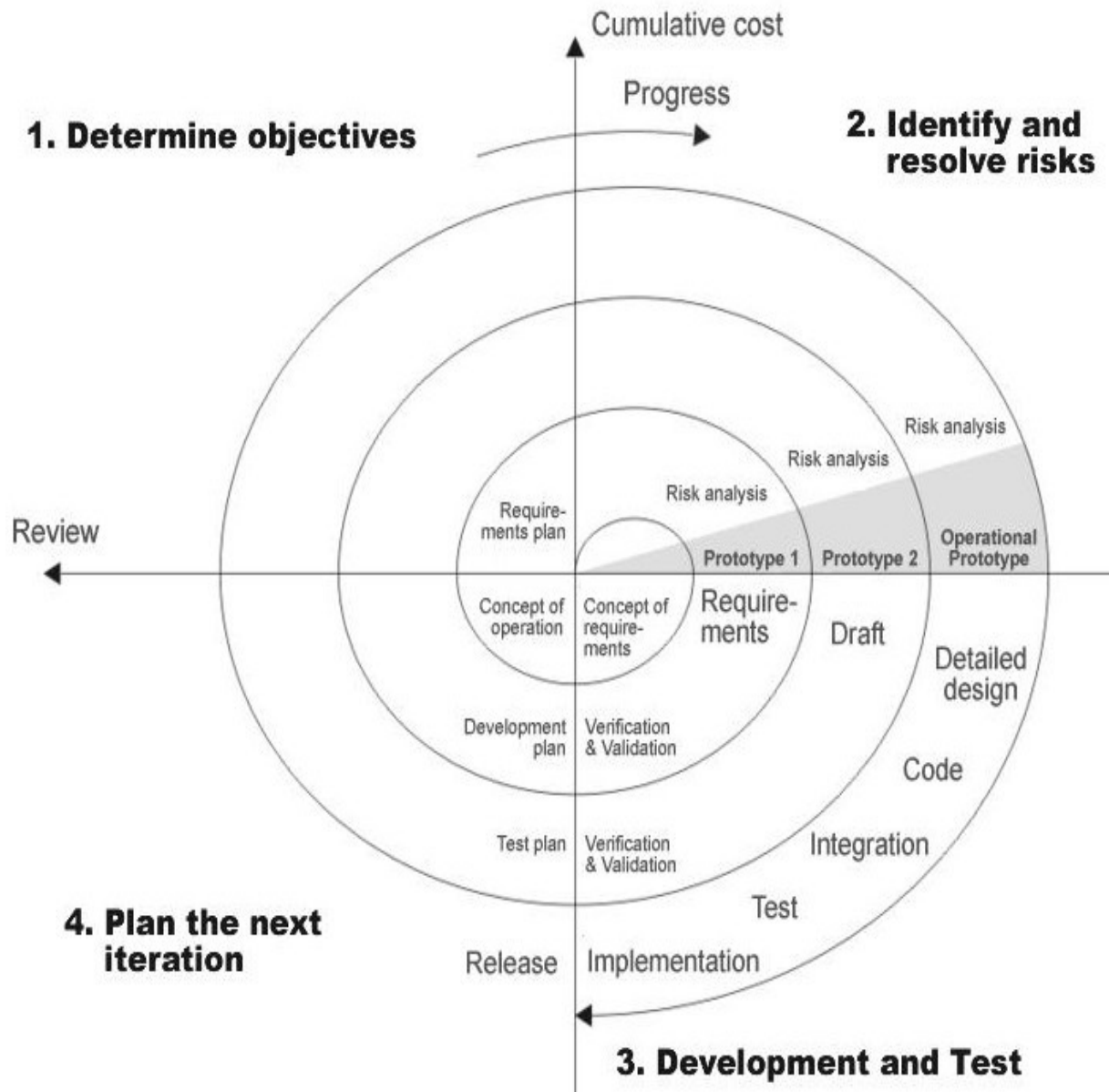
Fig 1.0-Spiral Model
