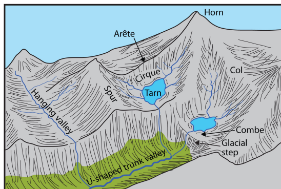
A. Schematic diagram of alpine glacial features
