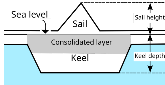
Figure 7: An idealized pressure ridge.
