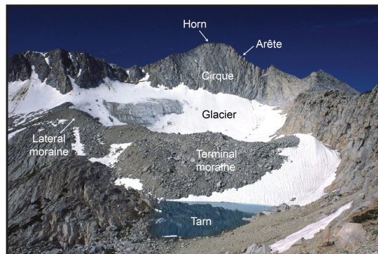
B. Glacial features on Mt. Conness
