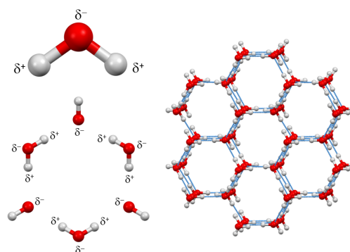
Figure 5: The crystal structure of "normal" hexagonal ice.
