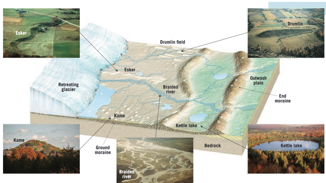
Figure 3: A retreating glacier with some common features.
