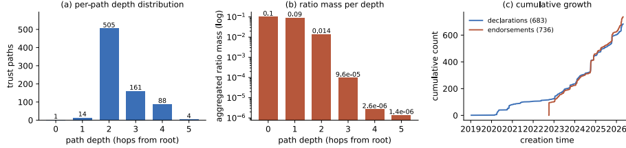
Fig. 2. (a) Per-path depth distribution. (b) Aggregated ratio mass per depth (log scale). (c) Cumulative growth of agent-key declarations and approved endorsements over time.
