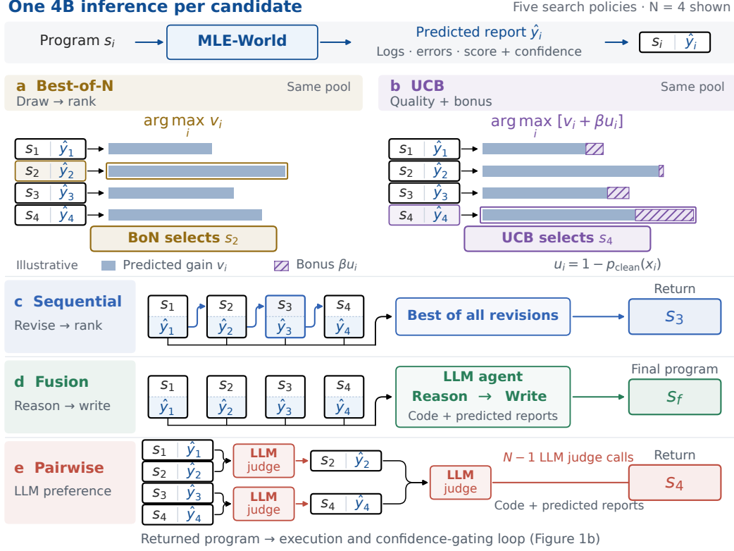
Figure 2: Five MLE-World search policies. Tiles show code s_i and predicted report \hat{y}_i ; x_i is the full input (Equation 1). UCB ranks by v_i + \beta u_i (Equation 4), where v_i = v(s_i) and u_i = u(x_i) . Illustrated with N = 4 usable predictions; each policy returns one program.
