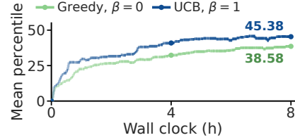
Figure 5: The exploration bonus improves over greedy. All other settings are fixed; only UCB’s \beta at Improve varies (Figure 8a).
