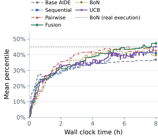
Figure 4: Search quality over time. Percentile of the validation-selected submission, carried forward and zero until valid. Dotted line: BoN (real execution)’s final mean (45.0%, 16 h cap). [Brian: Should we keep this figure? Without gating, UCB looks weak here (8 h: 45.1 vs. 47.2 for Fusion).]
