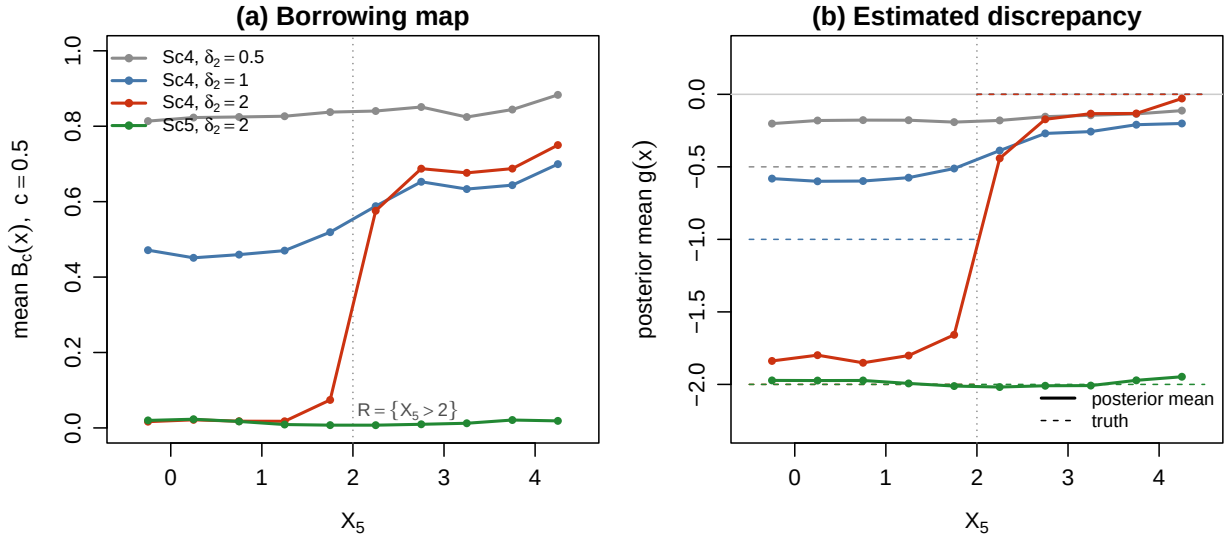
Figure 1: Regional and global shifts, Gaussian outcomes, LRC-BART (100): (a) the borrowing map \mathcal{B}_c(x) = P(|g(x)| < 0.5 | \text{data}) and (b) the posterior mean of g(x) , both averaged over the RCT control profiles in bins of width 0.5 on X_5 across the first 40 replicates. The RWD surface is raised by \delta_2 where X_5 \leq 2 (Sc4) or everywhere (Sc5), so the true discrepancy, dashed in (b), is -\delta_2 there.
