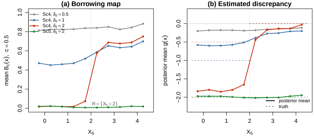
Figure 1: Regional and global shifts, Gaussian outcomes, LRC-BART (100): (a) the borrowing map \mathcal{B}_c(x) = P(|g(x)| < 0.5 | \text{data}) and (b) the posterior mean of g(x) , both averaged over the RCT control profiles in bins of width 0.5 on X_5 across the first 40 replicates. The RWD surface is raised by \delta_2 where X_5 \leq 2 (Sc4) or everywhere (Sc5), so the true discrepancy, dashed in (b), is -\delta_2 there.
