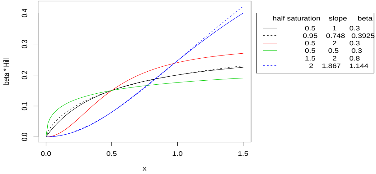
Figure 2: Hill functions.
