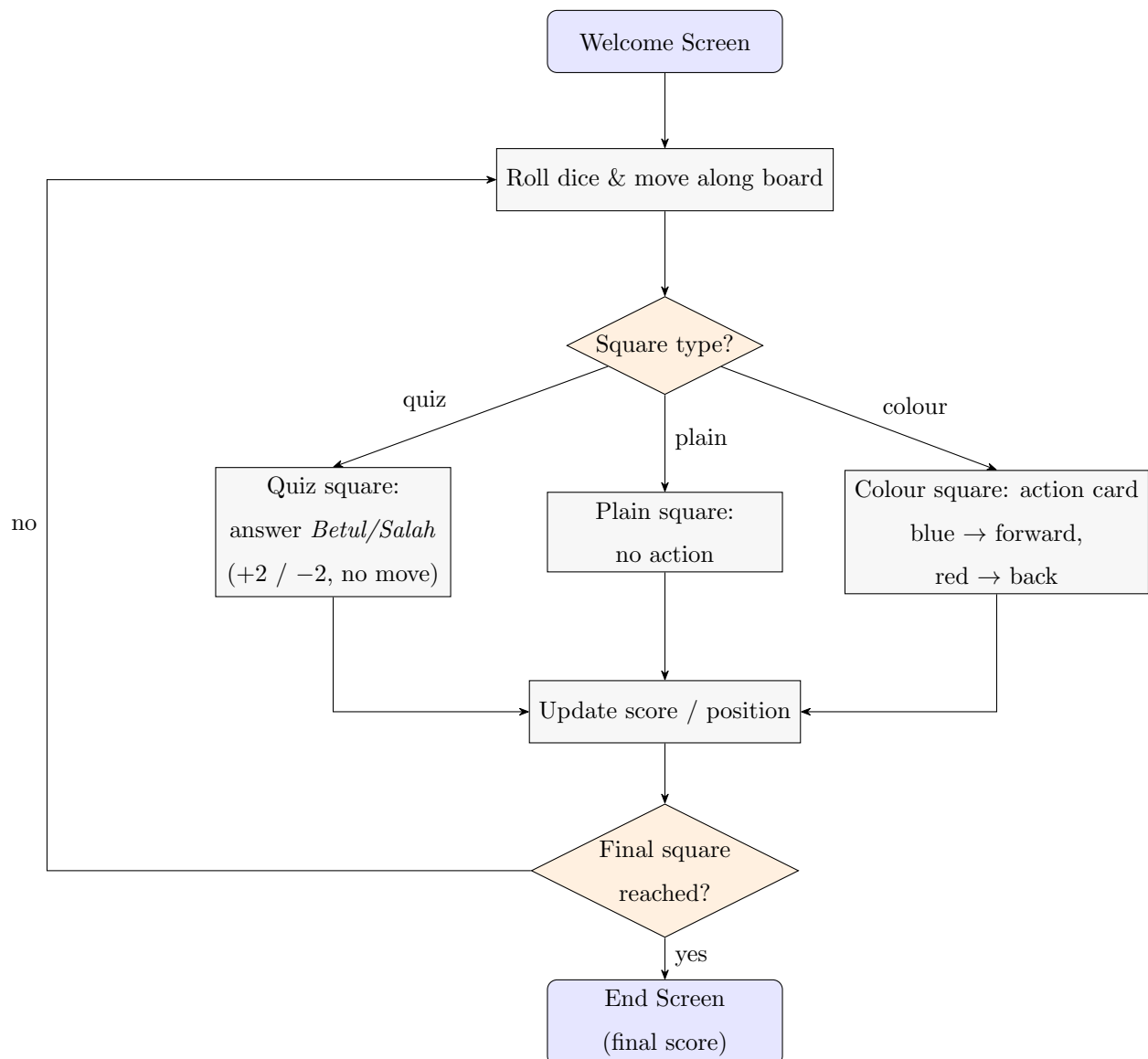
Figure 3: Game flow: each turn the player rolls the dice and moves, then acts on the square type — a plain square (no action), a Betul/Salah quiz square (score \pm 2 , no movement), or a colour-coded square (blue moves the player forward, red moves them back, after a short action card). The loop repeats until the final square is reached.
