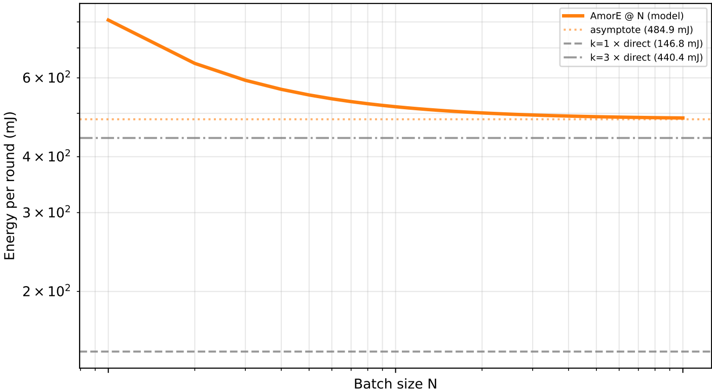
BLS12_381 — WITH_STOP (proposed: 0.5 \mu A during ServerWait) NO crossover in [1,100]
