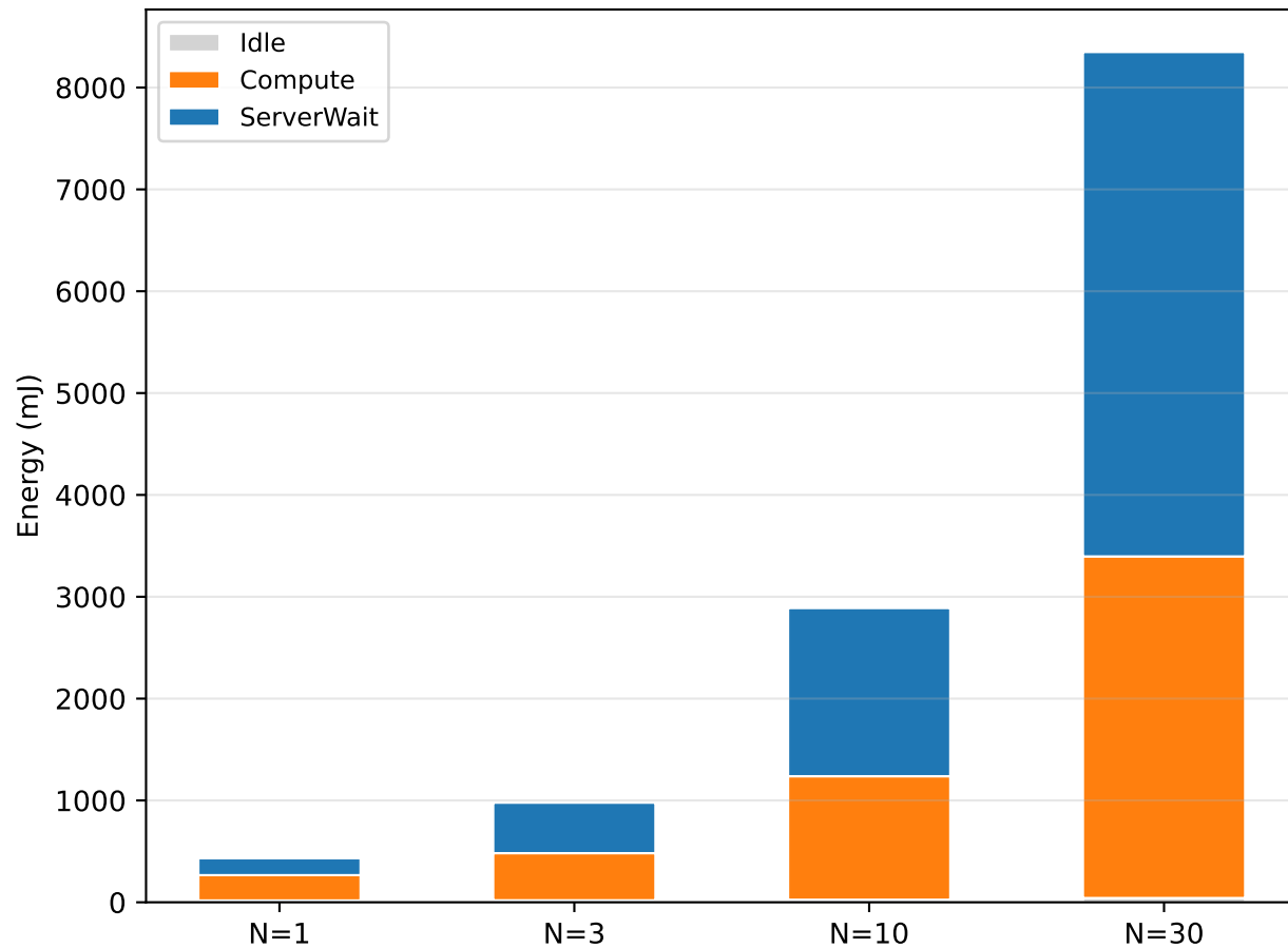
BN254 — energy breakdown by phase
