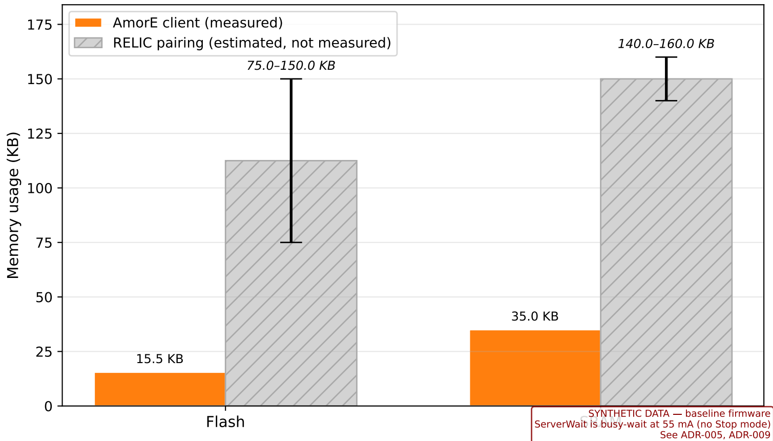
Figure 2b: Memory footprint — BLS12-381 AmorE measured; RELIC scaled from BN254 (12/8-limb), not built on this hardware
