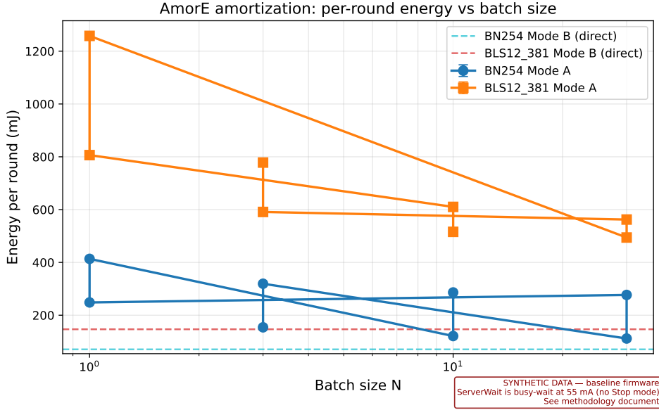
Figure 1: Energy per round vs batch size N . Mode A (AmorE) decreases by approximately 60 % from N=1 to N=30 for BN254 and by approximately 38 % over the same range for BLS12-381. Mode B (direct pairing) shows no N -dependence by construction; its level marks the per-pairing target AmorE is trying to undercut. Note that, under the baseline (busy-wait UART) firmware shown here, AmorE per-round energy remains above Mode B for all N in the measured range. See Section 5, subsection on crossover, for what changes that.
