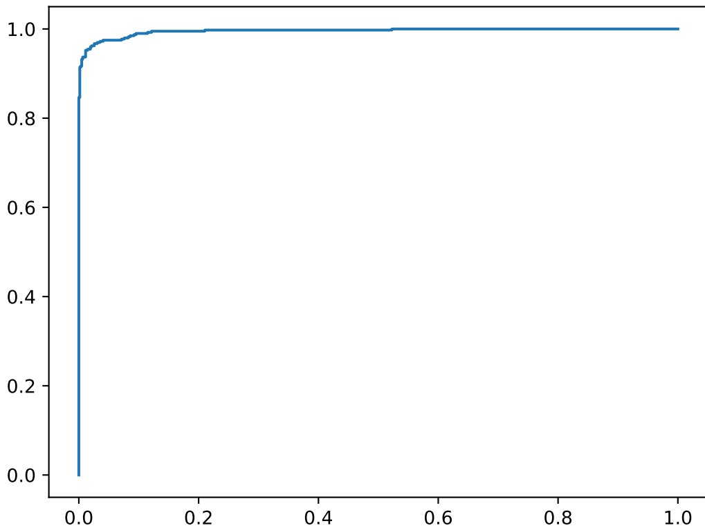
ROC Class 0
