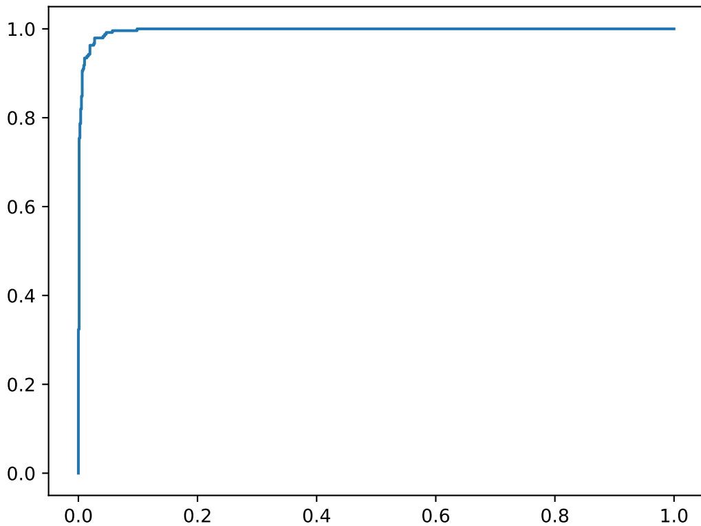
ROC Class 1
