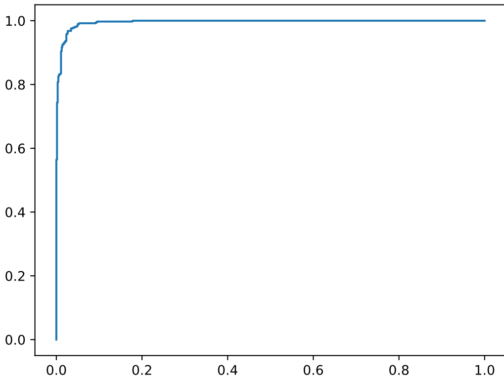
ROC Class 2
