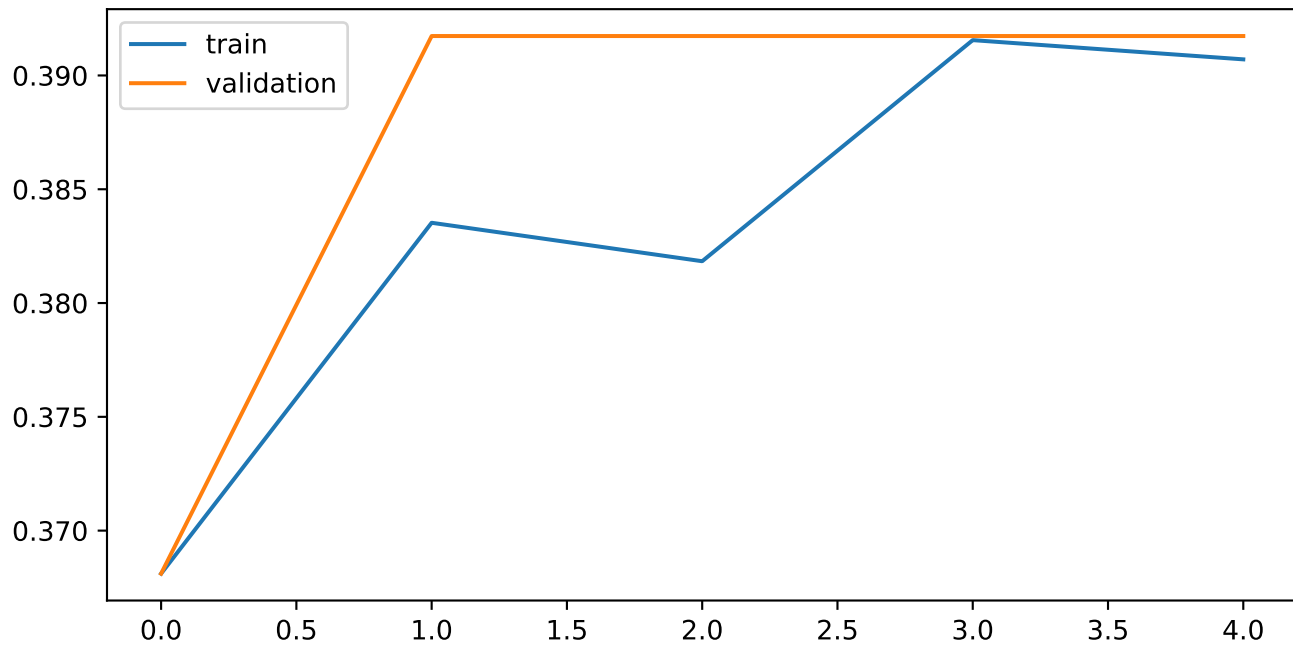
EfficientNetB0
