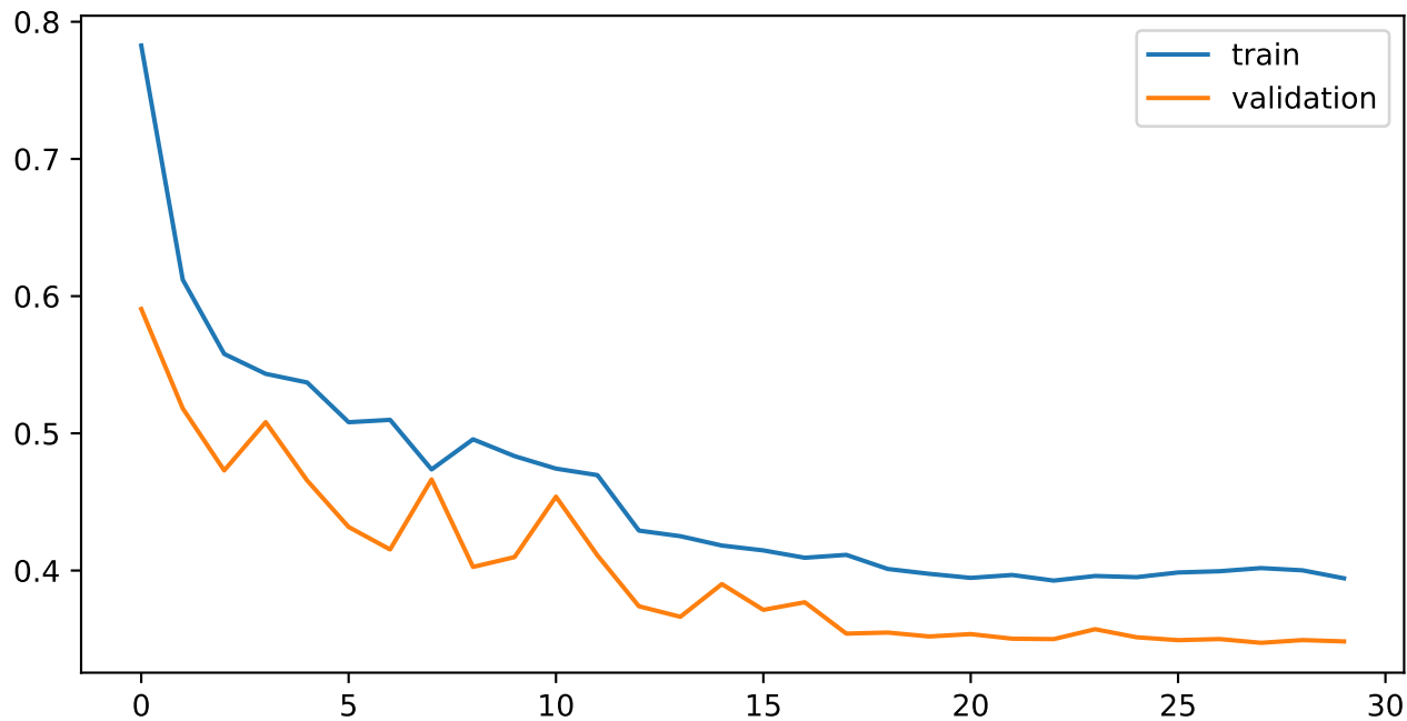
CustomCNN
