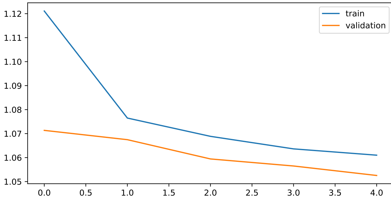
ResNet50
