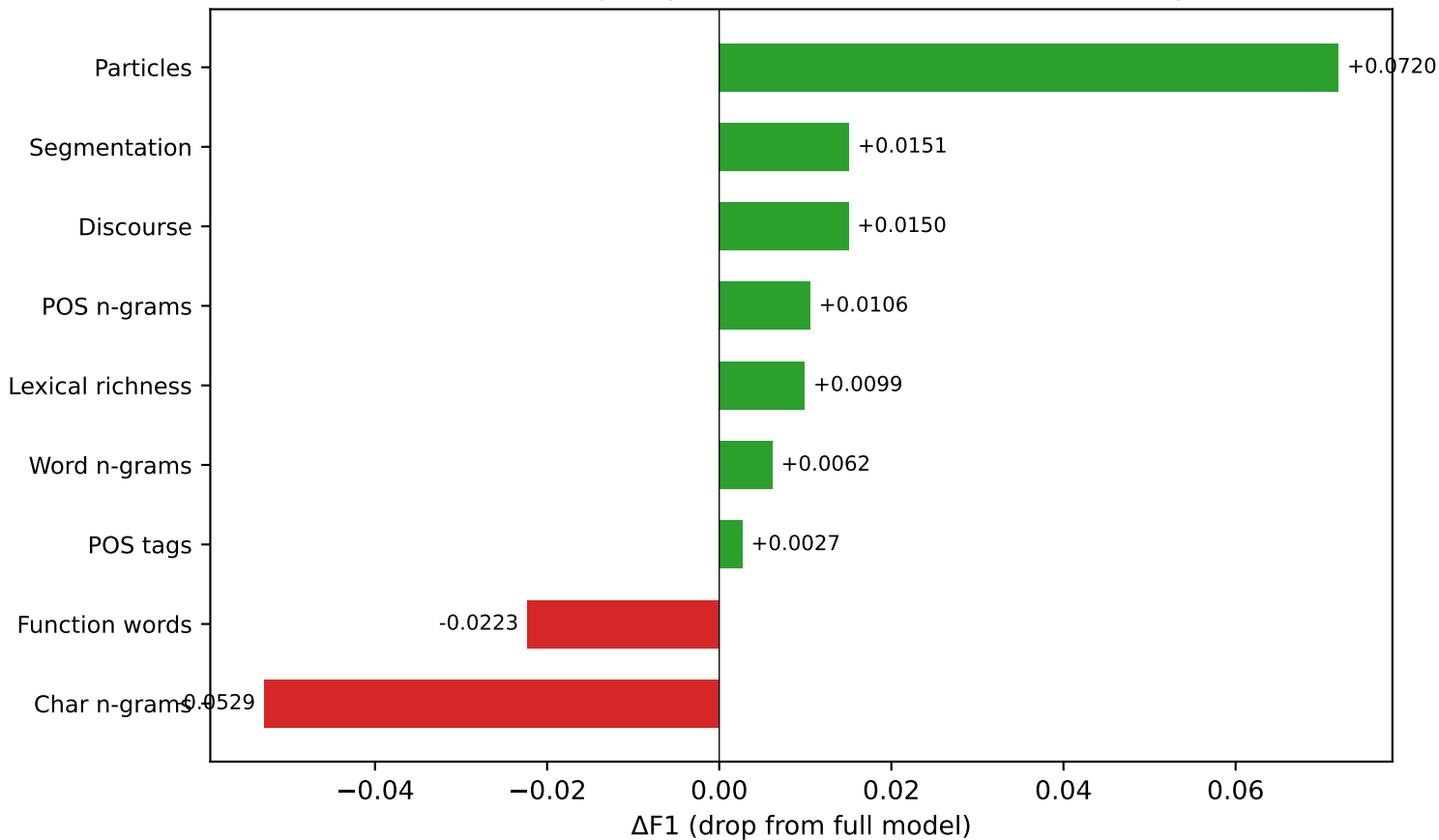
Feature Group Importance (Leave-One-Out F1 Drop)
