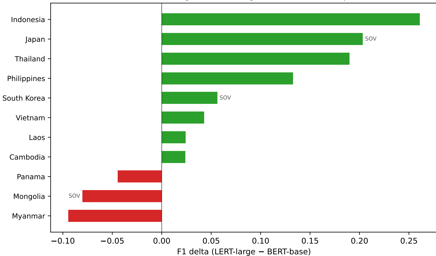
Per-L1 advantage of LERT-large over BERT-base (probe)
