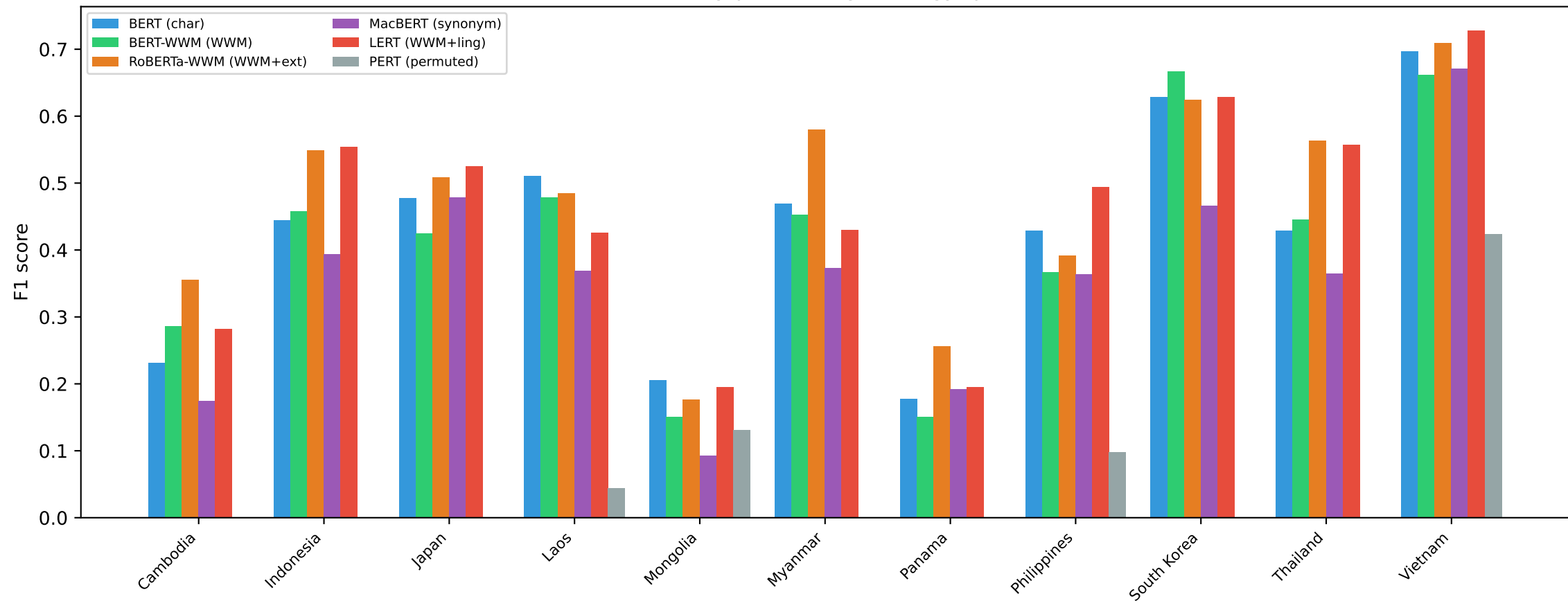
Per-L1 F1 by pretraining strategy (probes)
