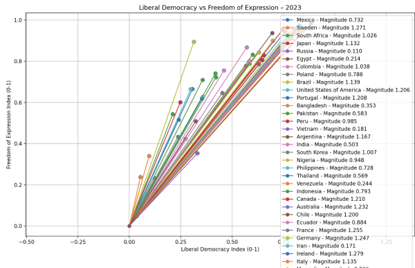
Figure 2: Liberal Democracy vs. Freedom of Expression from the V-Dem index for 2023
