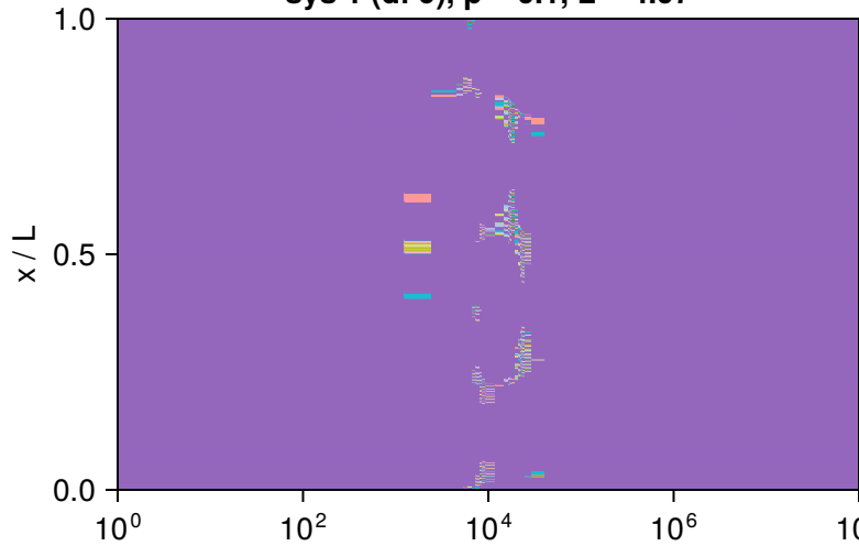
sys 1 (df 9), p = 1, L = 4.07
