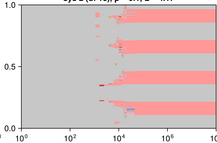
sys 2 (df 18), p = 1, L = 4.17
