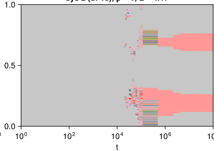
sys 2 (df 18), p = 1, L = 4.17
