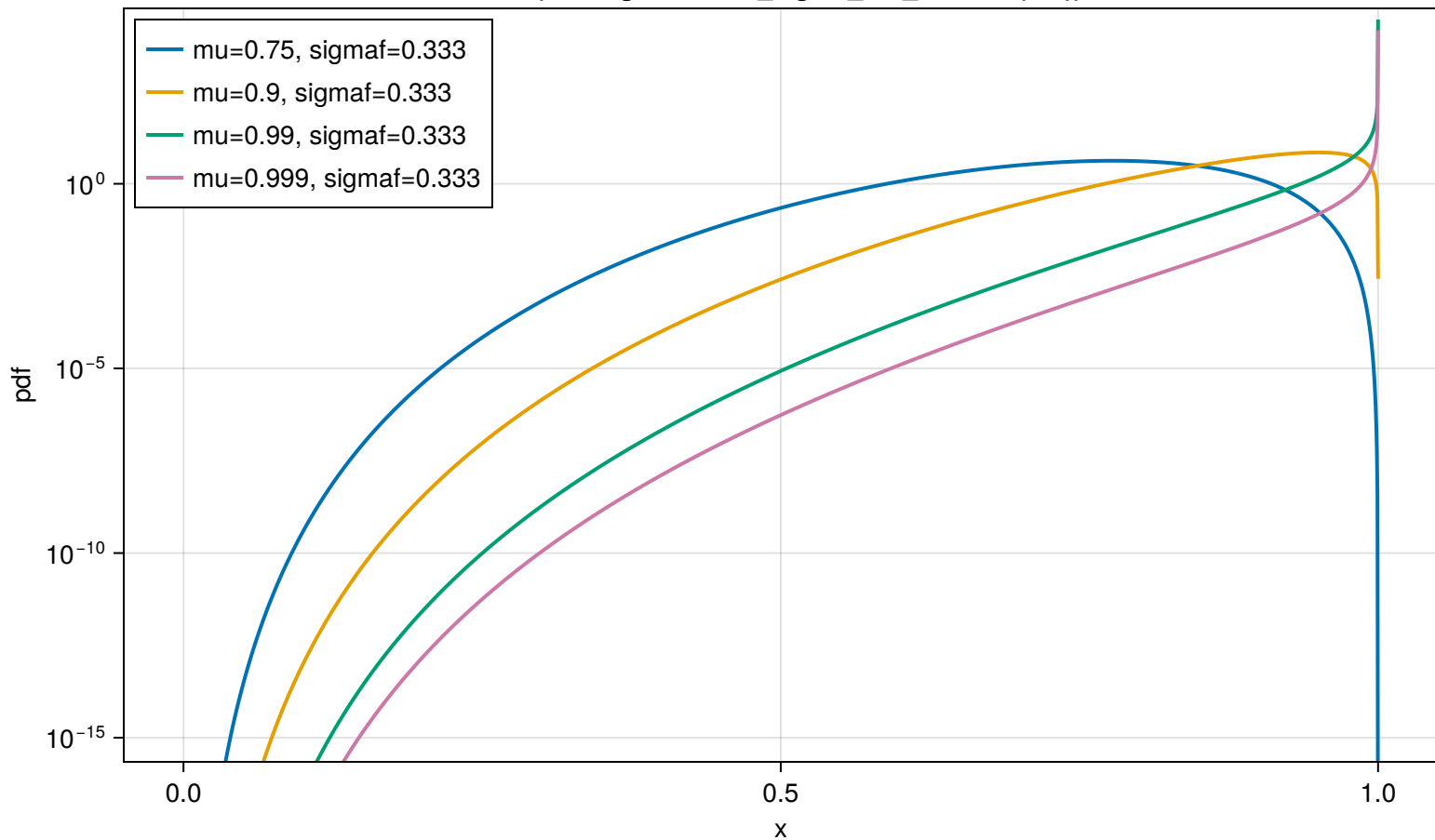
Beta( \mu , \sigma_{\text{maf}} * \text{max\_sigma\_not\_bimodal}(\mu) )
