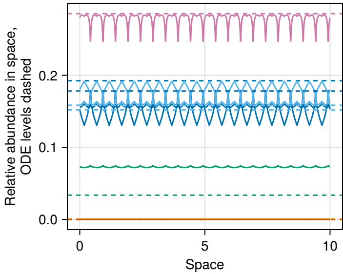
Comparing ODE vs PDE total abundances Community composition across space
