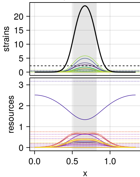
sys 14, p = 0.01 relamp 4.16, FWHM 0.24 L
