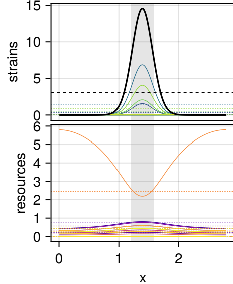
sys 24, p = 1 relamp 6.47, FWHM 0.14 L
