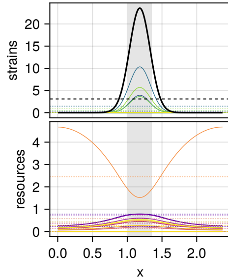
sys 24, p = 0.316 relamp 6.36, FWHM 0.15 L
