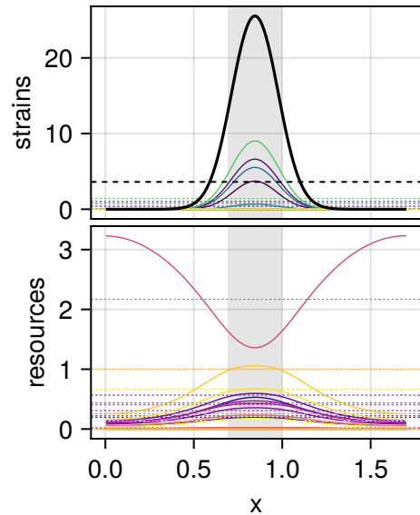
sys 40, p = 0.1 relamp 5.22, FWHM 0.18 L
