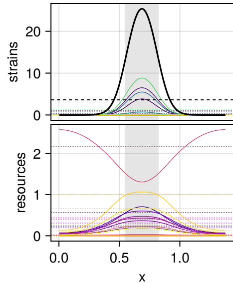
sys 40, p = 0.0316 relamp 4.61, FWHM 0.20 L
