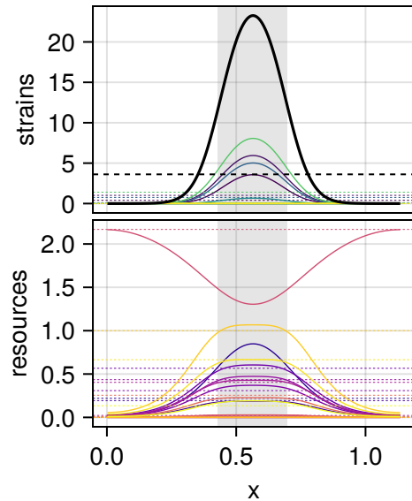
sys 40, p = 0.01 relamp 4.00, FWHM 0.24 L
