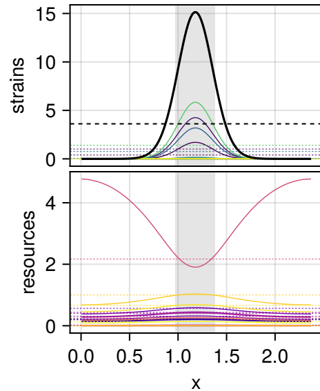
sys 40, p = 1 relamp 5.19, FWHM 0.18 L
