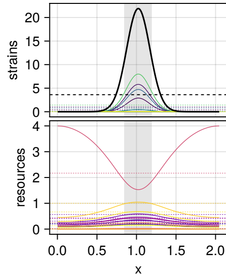
sys 40, p = 0.316 relamp 5.50, FWHM 0.17 L
