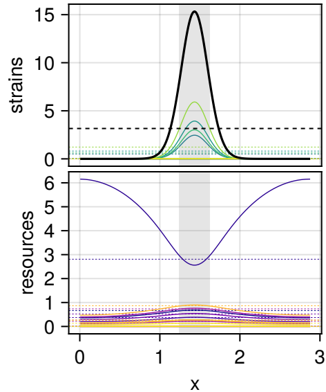
sys 97, p = 1 relamp 6.79, FWHM 0.14 L
