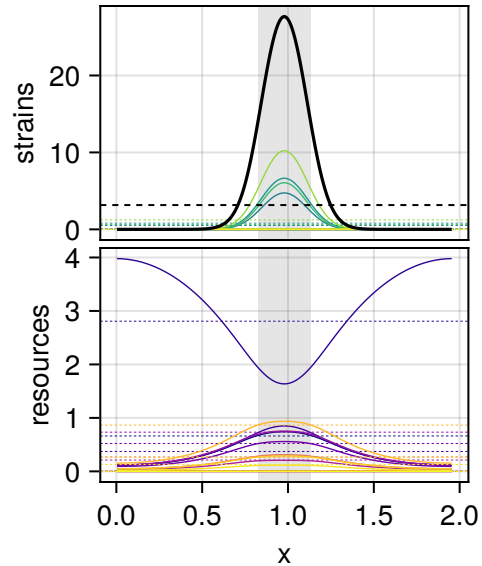
sys 97, p = 0.1 relamp 5.96, FWHM 0.16 L
