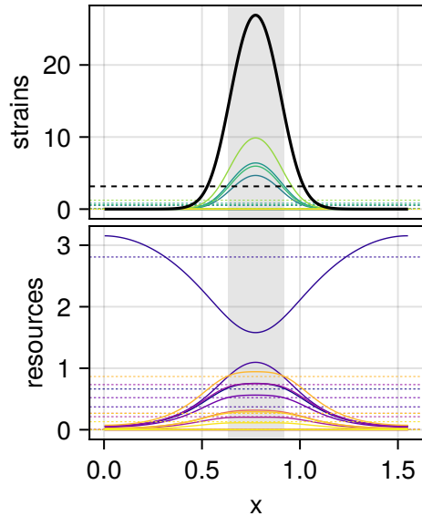
sys 97, p = 0.0316 relamp 5.10, FWHM 0.19 L
