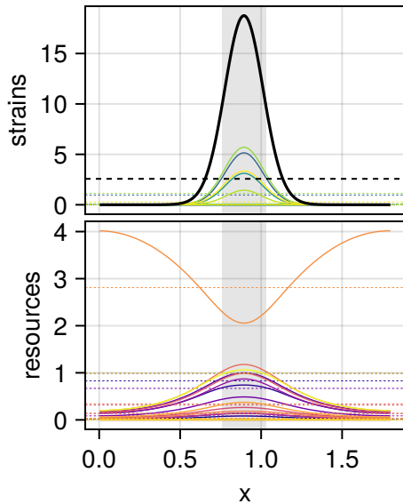
sys 46, p = 0.1 relamp 5.98, FWHM 0.16 L
