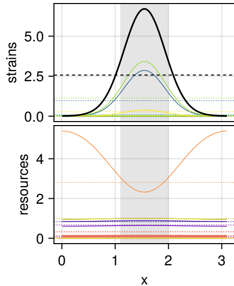
sys 46, p = 10 relamp 3.14, FWHM 0.30 L
