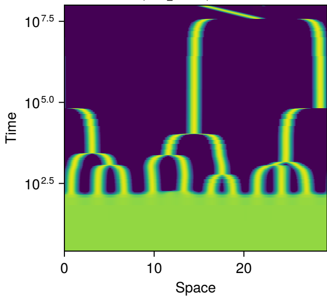
row 9, sys 5, p = 1 L = 29.3 , N_s = 6 Success, final_T 1e+08 , maxresid 1.0e-12
