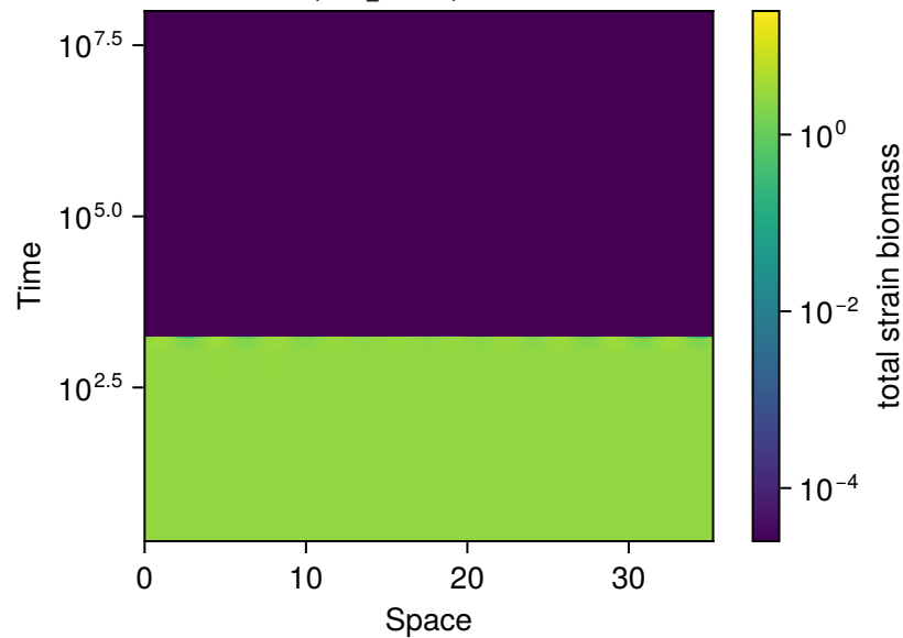
row 10, sys 5, p = 10 L = 35.2 , N_s = 6 Success, final_T 1e+08 , maxresid 2.2e-23
