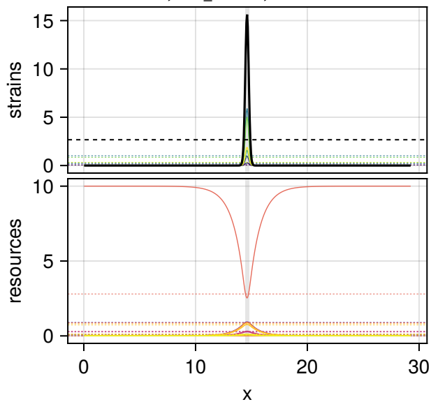
relamp 73.86, FWHM 0.01 L Success, final_T 1e+08 , maxresid 1.0e-12
