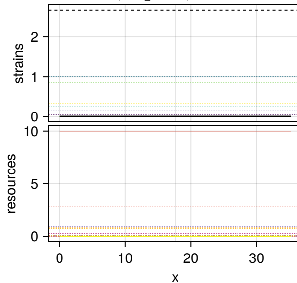
relamp 5.14, FWHM 0.01 L Success, final_T 1e+08 , maxresid 2.2e-23
