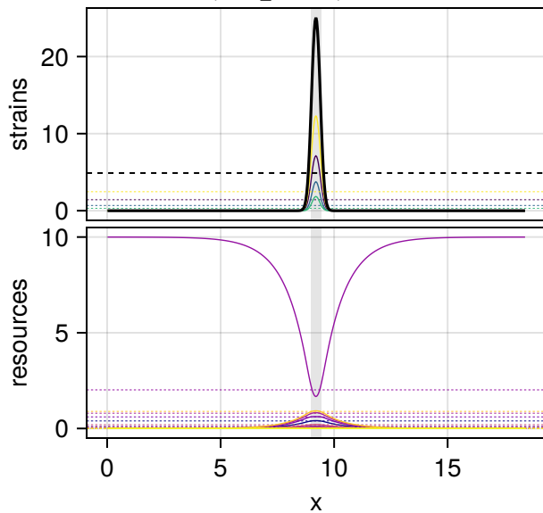
relamp 39.10, FWHM 0.03 L Success, final_T 1e+08 , maxresid 2.1e-12
