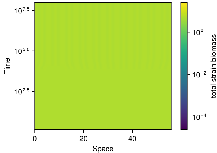
row 28, sys 14, p = 10 L = 56 , N_s = 4 Success, final_T 1e+08 , maxresid 2.2e-13
