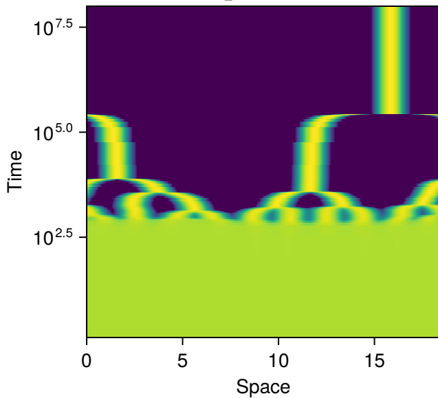
row 27, sys 14, p = 1 L = 18.4 , N_s = 4 Success, final_T 1e+08 , maxresid 2.1e-12
