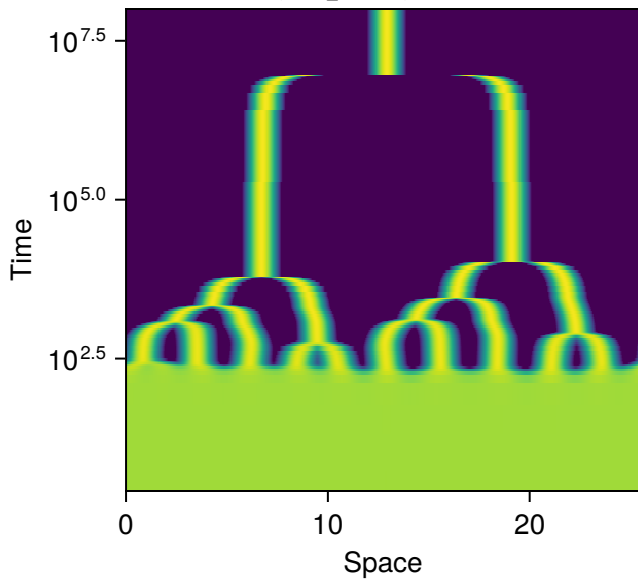
row 39, sys 20, p = 1 L = 25.5 , N_s = 7 Success, final_T 1e+08, maxresid 1.2e-12
