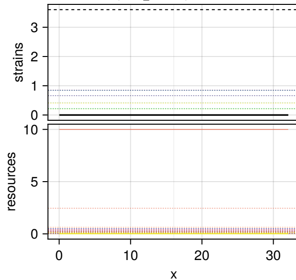
relamp 7.52, FWHM 0.00 L Success, final_T 1e+08, maxresid 3.0e-23
