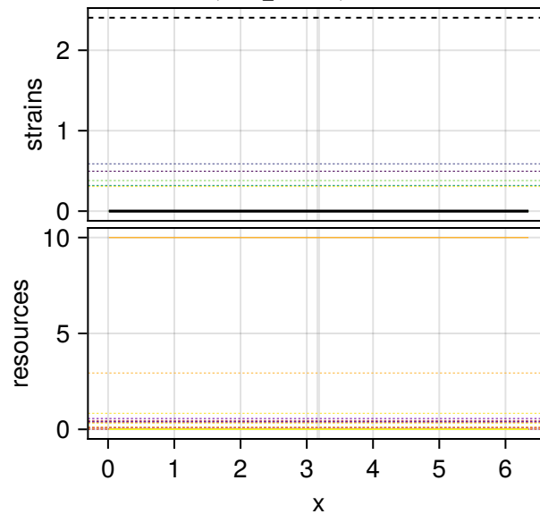
relamp 5.49, FWHM 0.01 L Success, final_T 1e+08 , maxresid 3.9e-25
