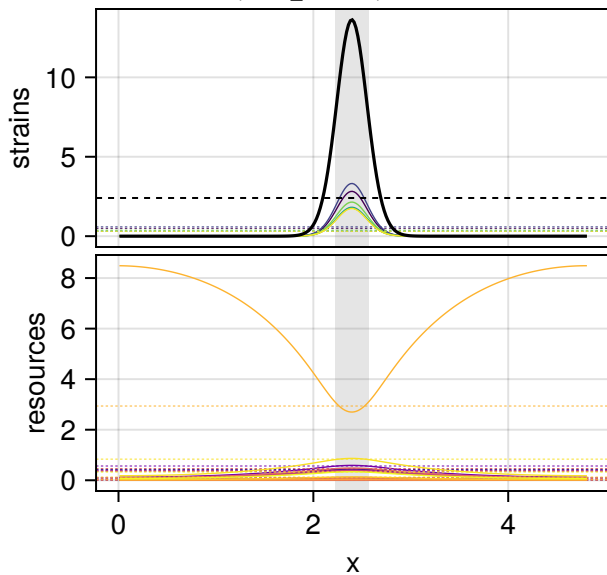
relamp 12.05, FWHM 0.08 L Success, final_T 1e+08 , maxresid 7.8e-12
