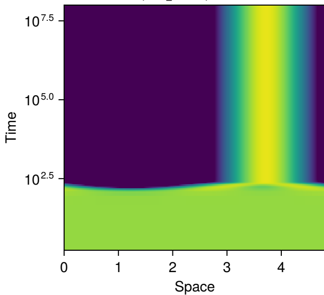
row 5, sys 3, p = 1 L = 4.82 , N_s = 6 Success, final_T 1e+08 , maxresid 7.8e-12
