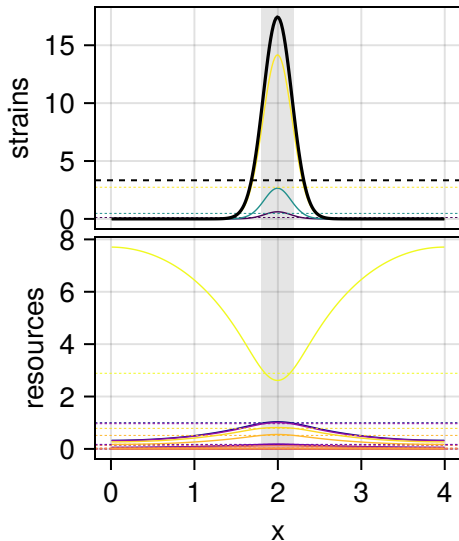
row 3, sys 2, p = 1 relamp 9.25, FWHM 0.10 L Success, final_T 1e+08, maxresid 8.7e-11
