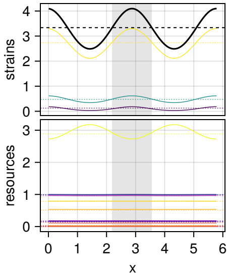
row 4, sys 2, p = 10 relamp 0.49, FWHM 0.24 L Success, final_T 1e+08, maxresid 4.0e-12
