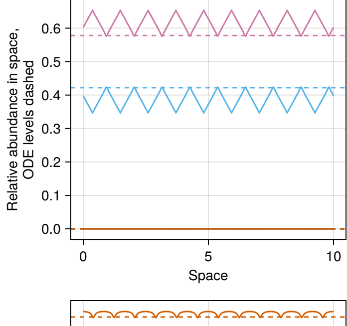
Community composition across space
