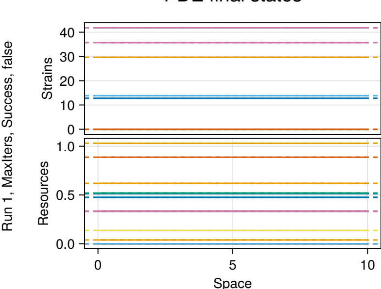
PDE final states
