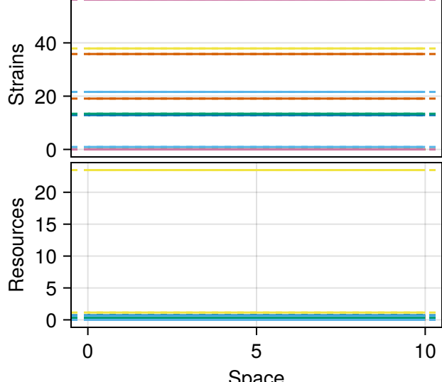
PDE final states
