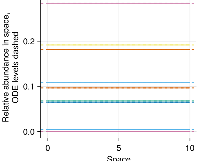
Community composition across space
