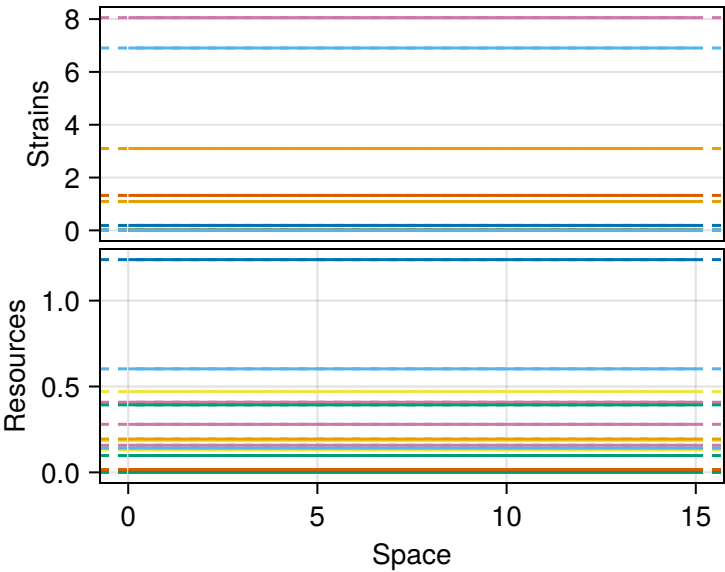
PDE final states
